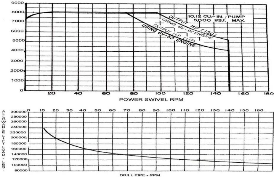
PERFORMANCE DATA, BOWEN S-3.5 POWER SWIVEL
